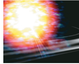
orbit
