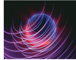
radiation
